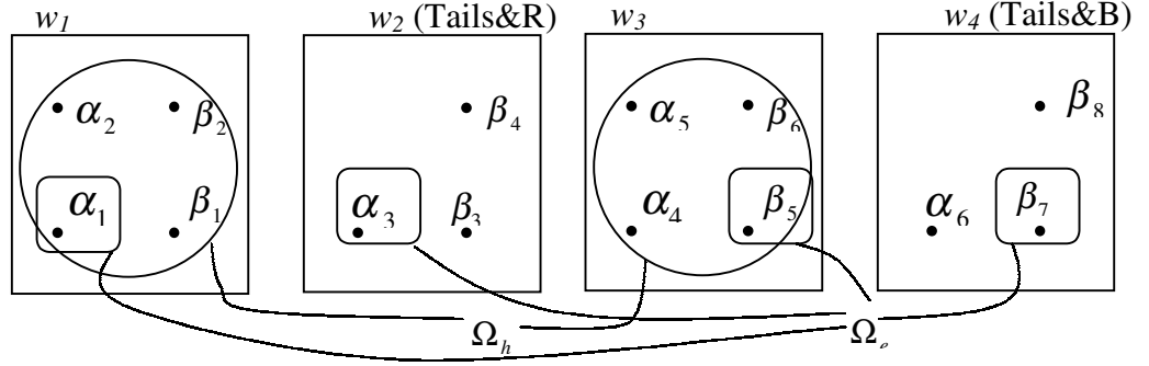
Figure 8: Modeling God's Coin Toss using SSSA-R with minimal reference class ( R = R^0 )
