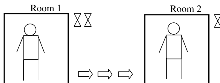
Figure 4: One observer spending different amounts of time in two rooms
