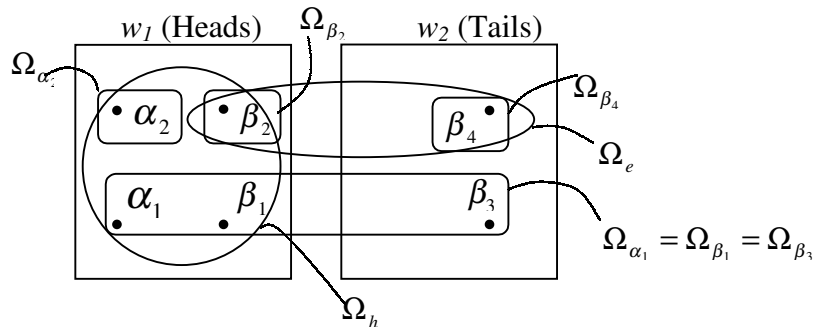
Figure 7: SSSA-R applied to God's Coin Toss, revised approach
