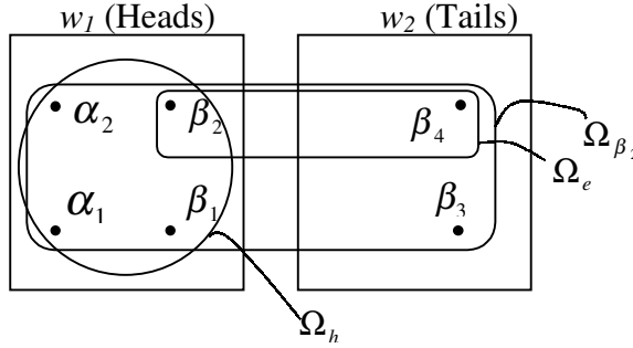
Figure 6: SSSA-R applied to God's Coin Toss using R = R^U (original approach)
